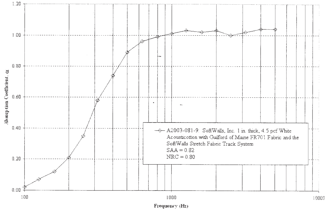
Graph 1. Sound Absorption Performance of SoftWalls, Inc. 1 in. thick, 4.5 pcf Acousticotton with Guilford of Maine FR701 Fabric and the SoftWalls, Inc. Stretch Fabric Track System
